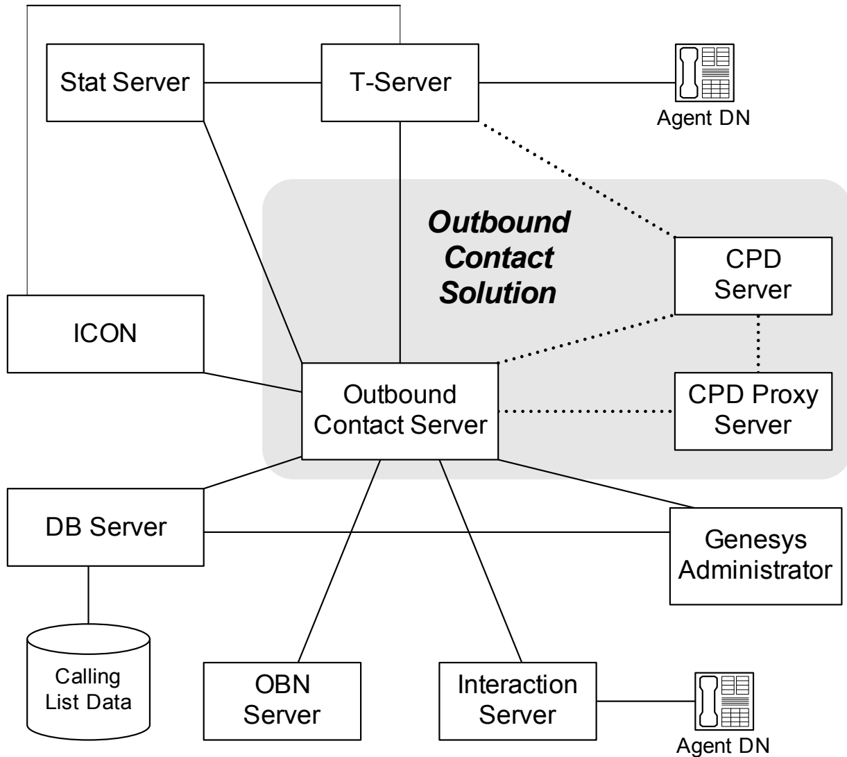
Figure 1: Outbound Contact Architecture - T-Server Configuration
